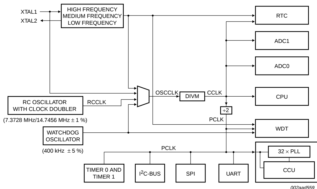
Fig 5. Block diagram of oscillator control
