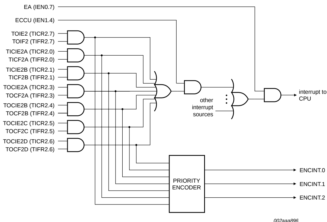
Fig 10. Capture/compare unit interrupts
