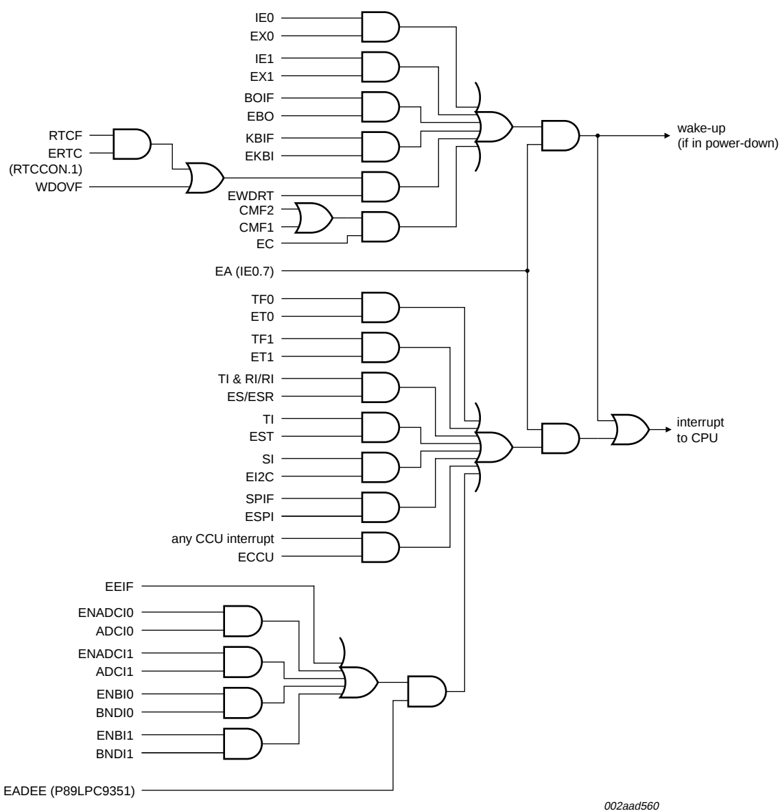
Fig 6. Interrupt sources, interrupt enables, and power-down wake-up sources
