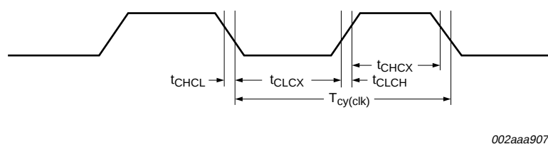
Fig 22. External clock timing (with an amplitude of at least V_{i(RMS)} = 200 mV)
